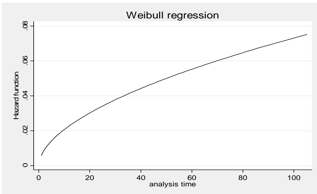
FIGURE 2. ESTIMATED HAZARD BASED ON WEIBULL REGRESSION
